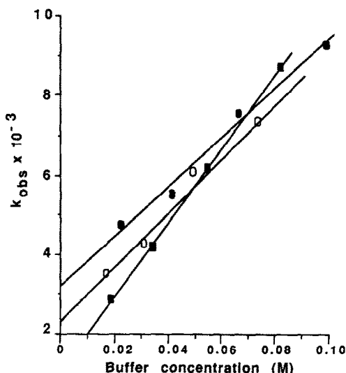
Fig. 5. Effect of the buffer concentration on the degradation of PC in citrate buffer at 72°C. (●, pH 5.0; ○, pH 5.5; □, pH 6.0). The lines were calculated by linear regression analysis. Each point represents the mean of at least two separate determinations.
